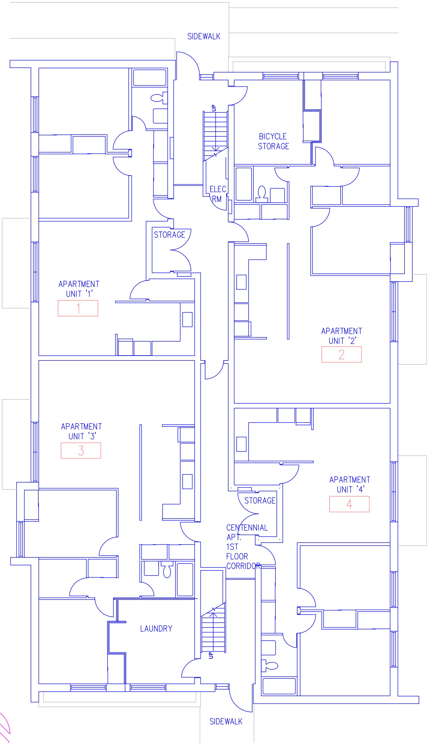
CENTENNIAL APARTMENTS – 1ST FLOOR
